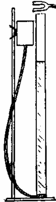
Figure 2. The resonance tube apparatus.
